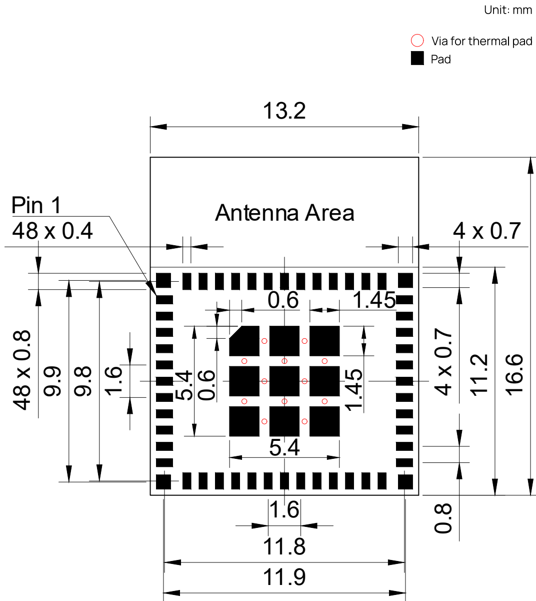
Figure 2: Shelly MOD1 Recommended PCB Land Pattern
